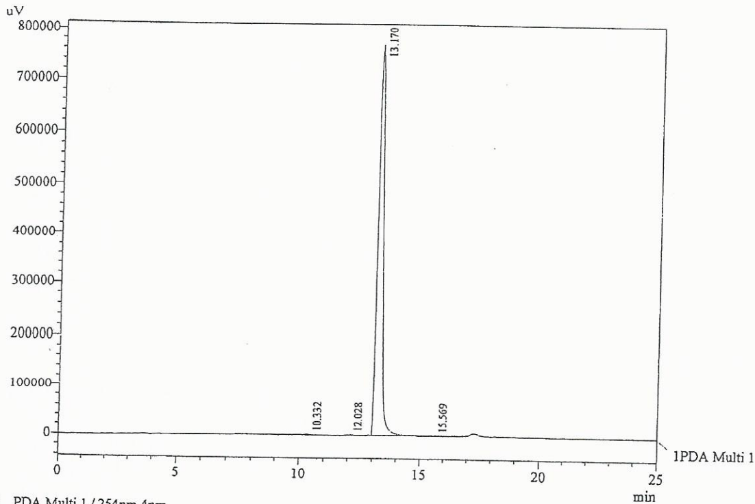
Chromatogram
